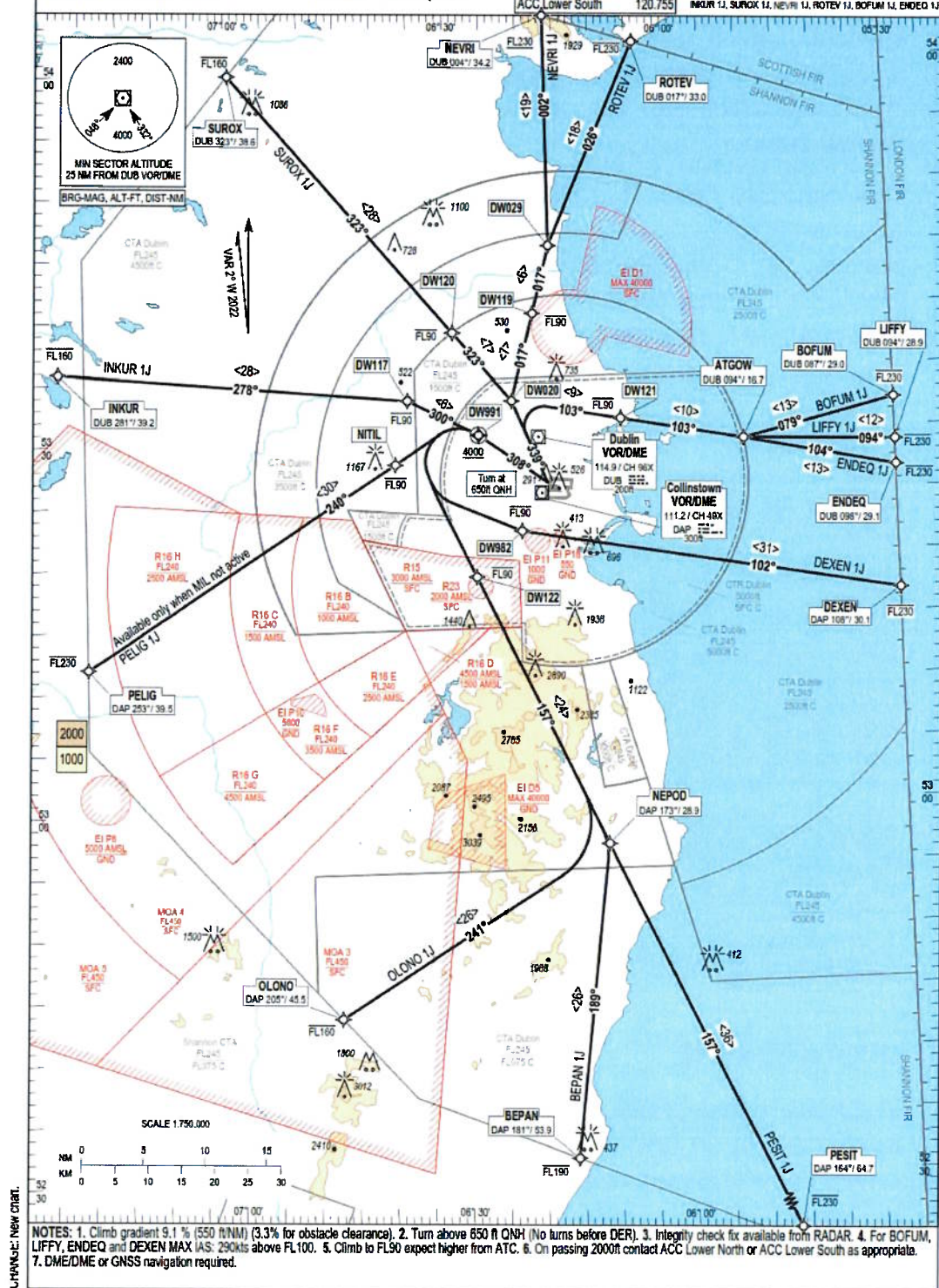
Figure 3 SID For North Runway Westerly Departures
